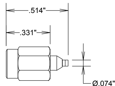
SMA-M U.FL/JACK
