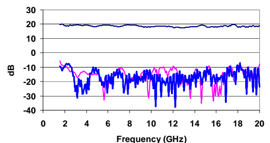
Gain and Return Loss
