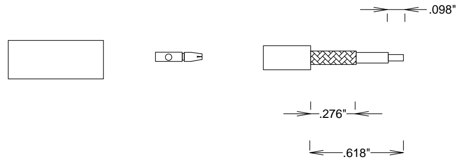
STRIPPING DIMENSIONS
