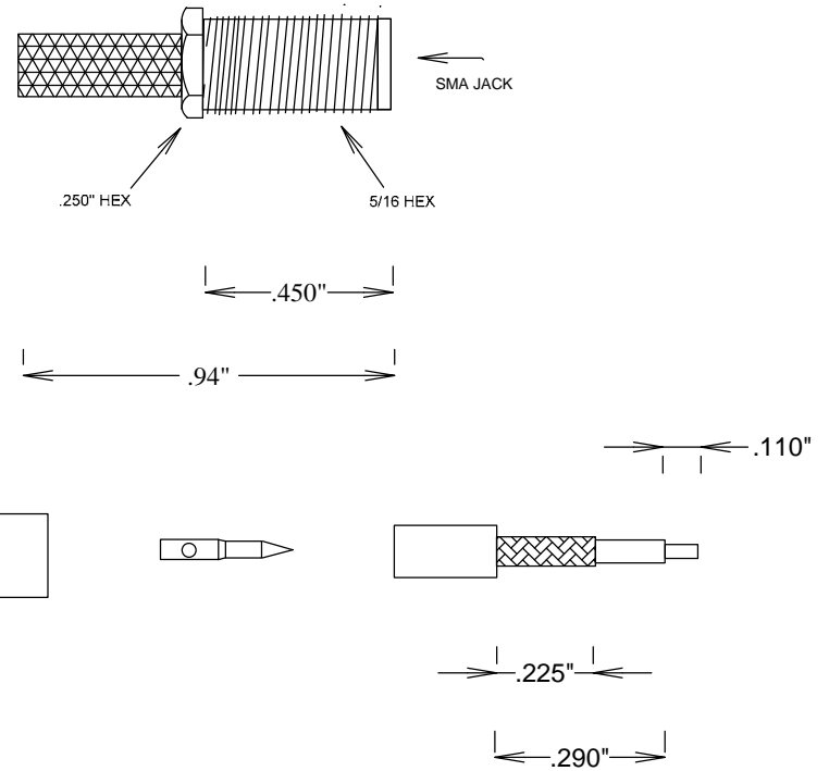
STRIPPING DIMENSIONS
