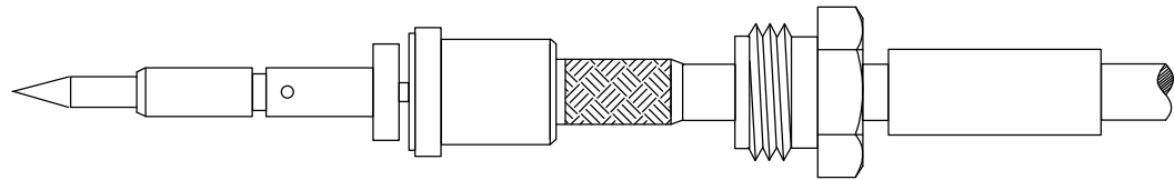
Component positioning before inserting pin into connector
