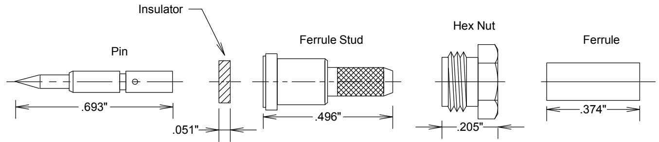
Component positioning before inserting pin into connector
