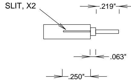
STRIPPING DIMENSIONS
