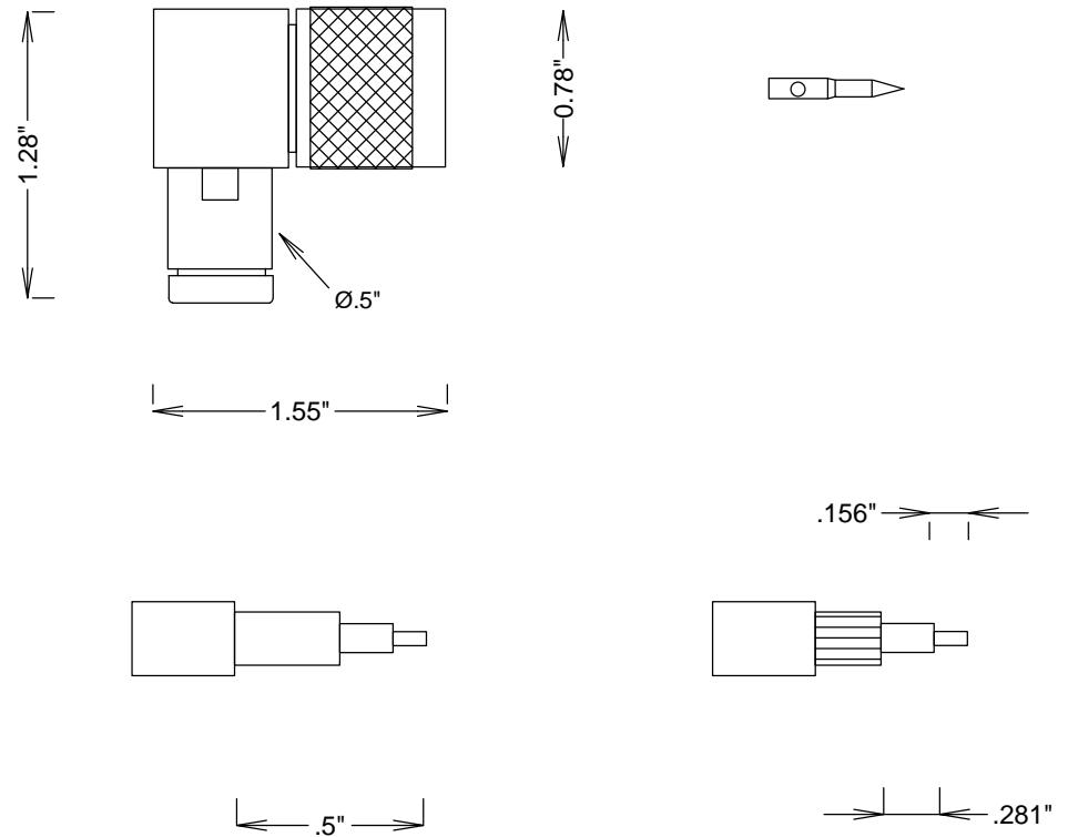
STRIPPING DIMENSIONS
