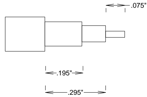
STRIPPING DIMENSIONS
